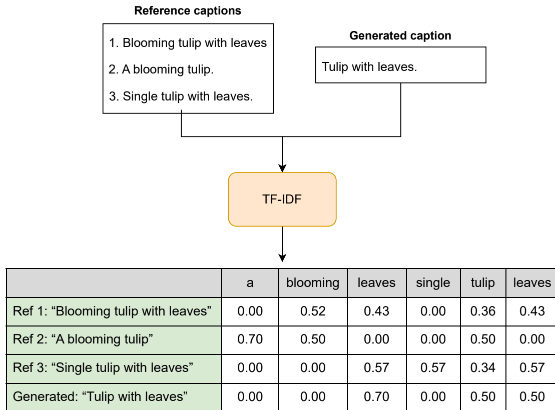
Figure 15: TF-IDF converting captions to numerical representations
