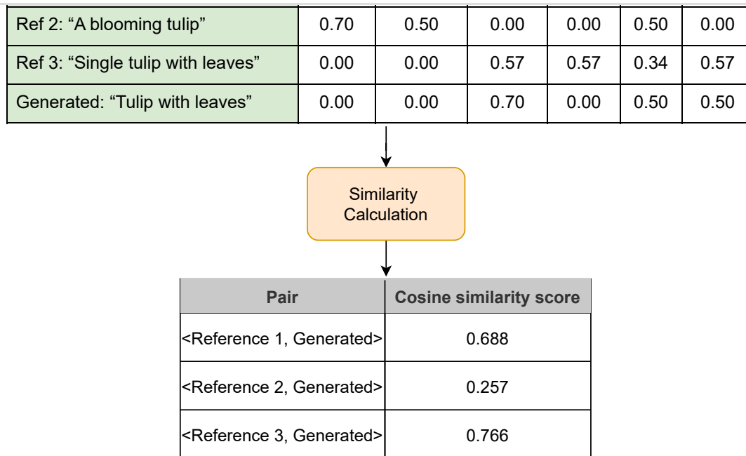
Figure 16: Calculation of cosine similarity between generated and reference captions
