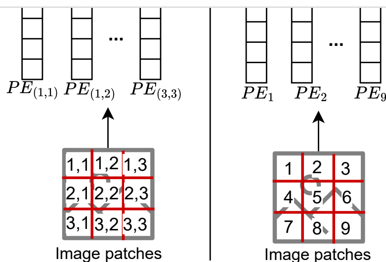
Figure 10: 1D vs. 2D positional encoding
