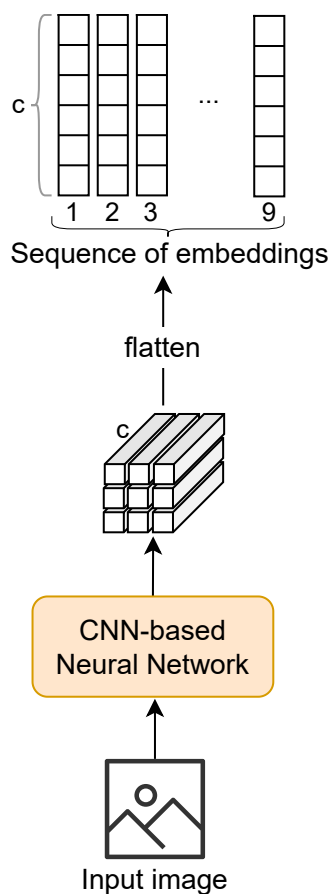
Figure 7: A CNN-based image encoding
